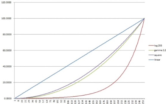
Dimming Curve
