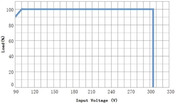
Derating Curve
